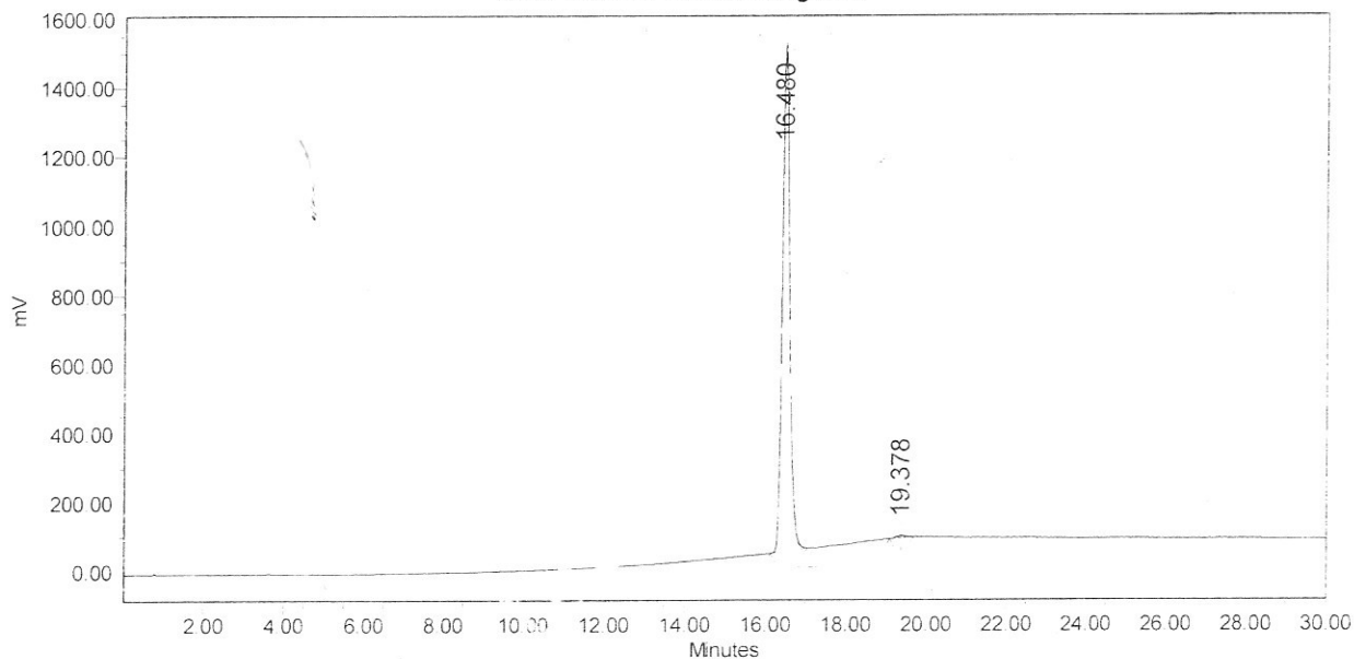
Auto-Scaled Chromatogram
